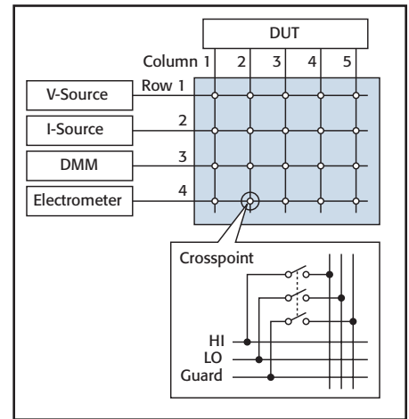
Figure 3. Matrix Switch
