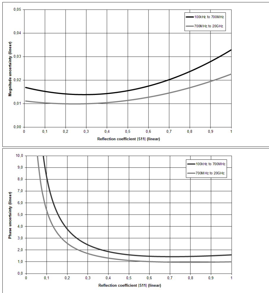
Typical accuracy of reflection magnitude and reflection phase measurements for the R&S ® ZNBT20 in the frequency range from 100 kHz to 20 GHz. Analysis conditions: S_{12} = S_{21} = 0 , cal. power -10 dBm, meas. power -10 dBm.
