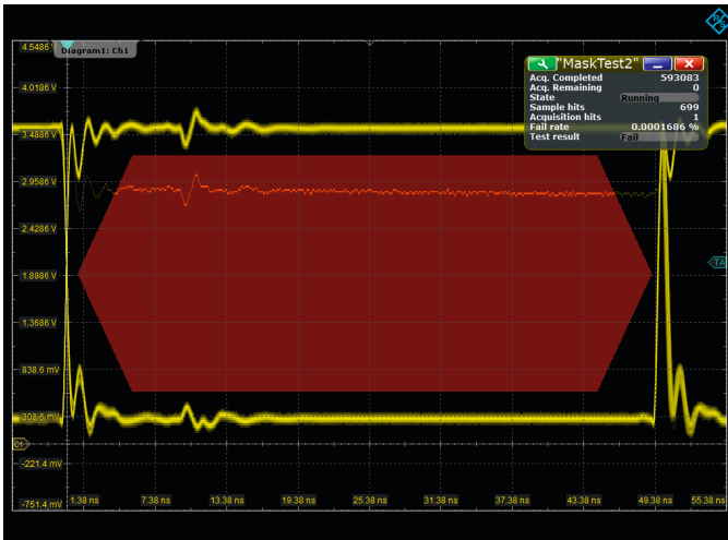
R&S®RTE masks consist of up to eight segments. Hardware implementation keeps the acquisition rate high, and mask violations are quickly found.
