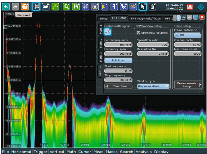
The R&S®RTE FFT function offers accuracy, speed, functionality and ease of use.
