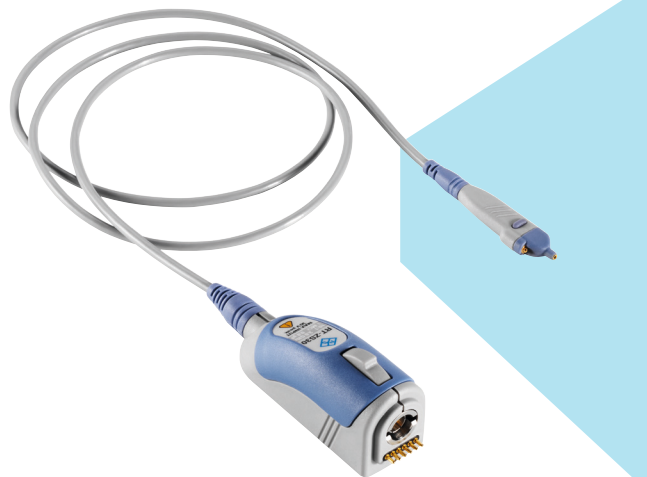
Rohde & Schwarz active probes (1.0 GHz to 6.0 GHz).
