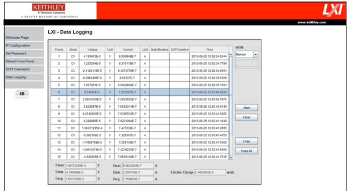
Figure 9. Web page display of the LXI-data logging function showing all parameters stored and the associated statistics.
