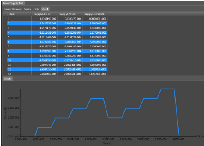
Figure 11. KickStart plot with measurement table.
