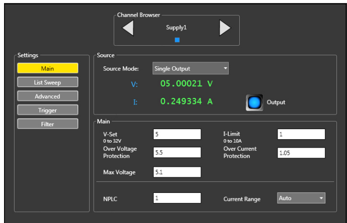
Figure 10. KickStart DC power main screen.
