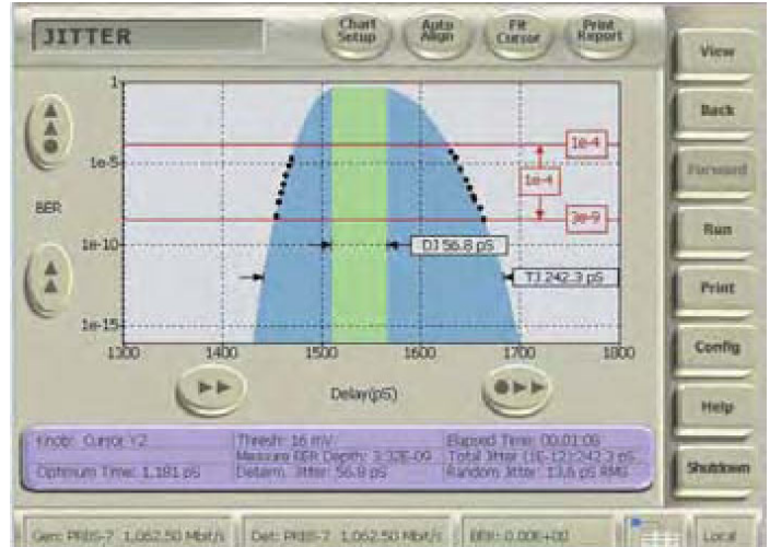
To get better results, BER data above 1e-4 BER are not used when predicting deep BER values. The longer the test runs, the more precise the measurements become.
