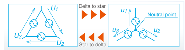
Δ-Y conversion
